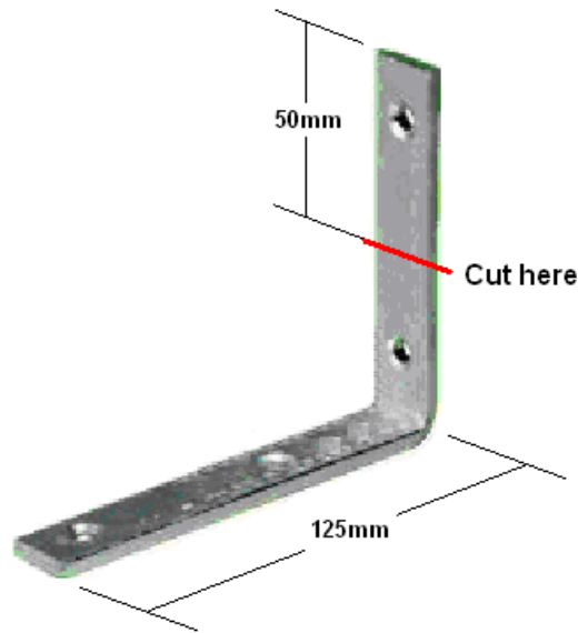
Figure 12 Mounting Brackets
