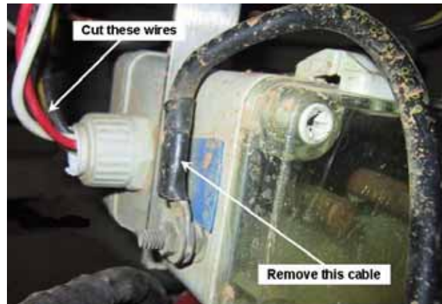
Figure 3 Black Earth Cable to be Disconnected and Wires to Cut
