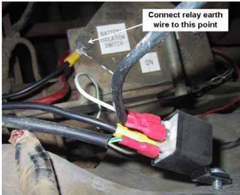
Figure 9 New Relay Ground Connection Point
