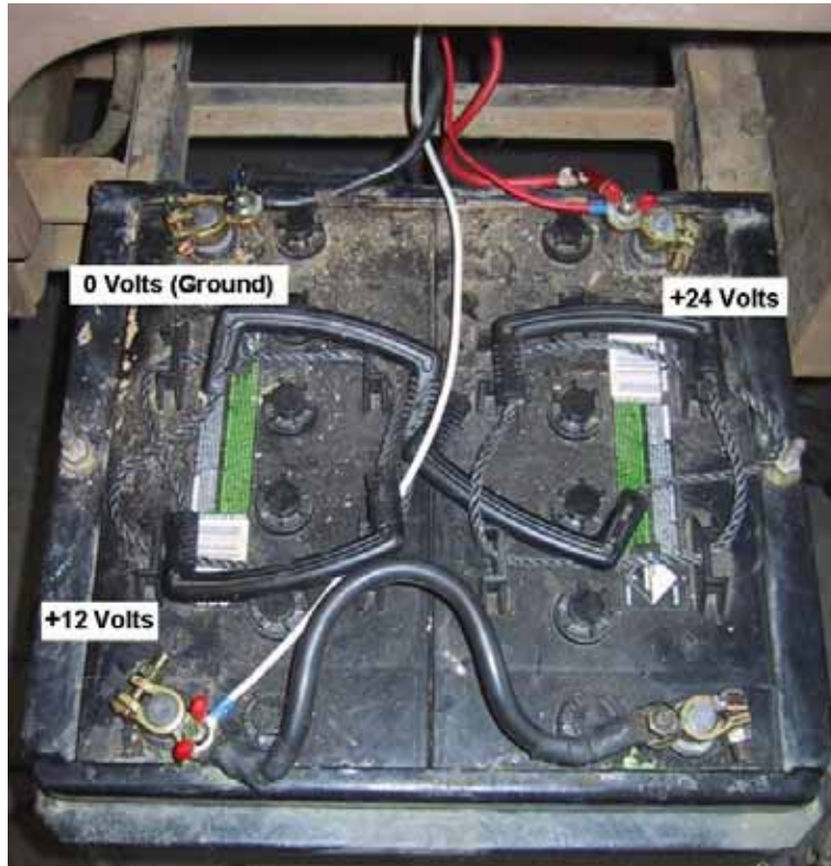
Figure 16 Module Battery Connections
