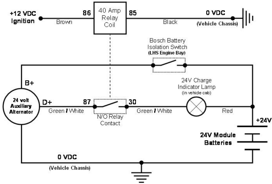
Figure 5 24-volt Auxiliary Alternator Charge Indicator Lamp Relay Circuit
