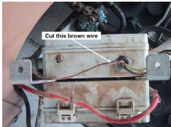
Figure 4 12-volt Vehicle Ignition System Wire
