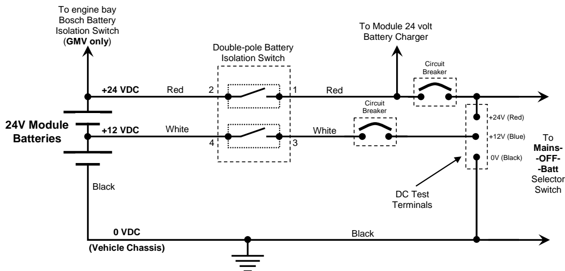
Figure 10 Wiring Diagram Showing the New Module Battery Isolation Switch
