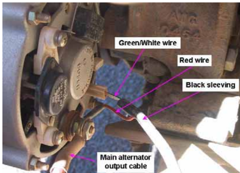
Figure 8 24-volt Auxiliary Alternator Connections
