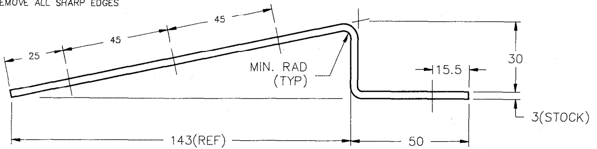
FIG 2 - BUTT BOX SUPPORT BRACKET AUSTSTEYR (MACK ALL TYPES)
