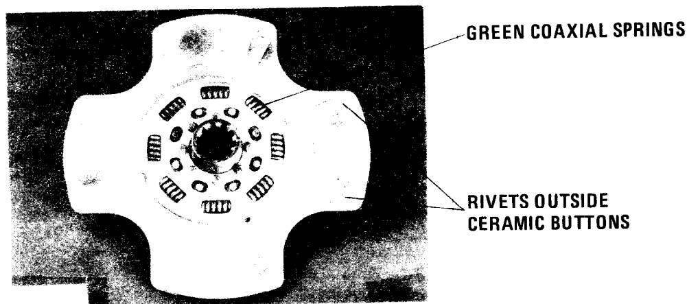
FIG 1 - REPLACEMENT CLUTCH DISC IDENTIFICATION
